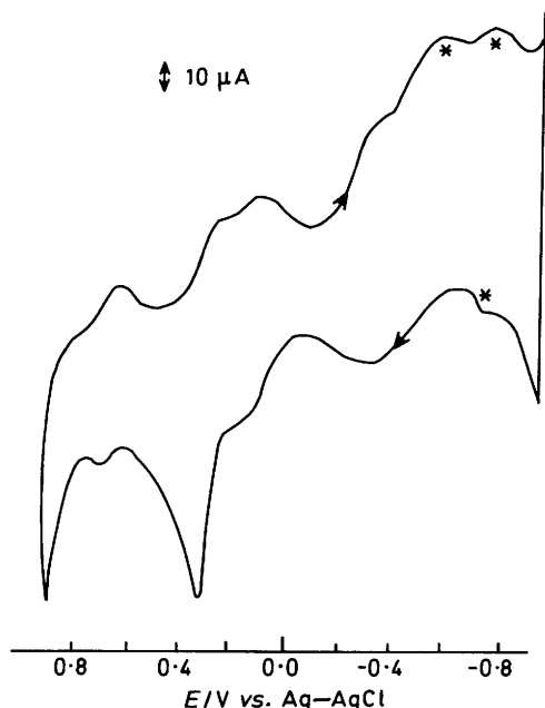
Figure 3. Cyclic voltammogram of 10^{-3} mol \text{dm}^{-3} trans -[RuO 2 (HIO 6 ) 2 ] 6- in an aqueous solution of 0.1 mol \text{dm}^{-3} KCl (pH 10.8) using platinum electrodes and scan rate of 50 mV \text{s}^{-1} . * Denote irreversible periodate peaks slightly shifted cathodically by 0.01–0.05 V compared to the free ligand, at the same concentration and pH at 25 °C
